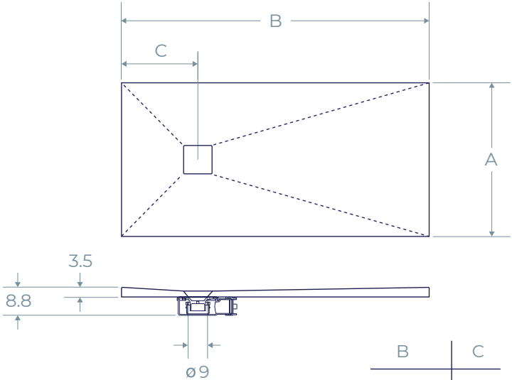
1 Plan and elevation (cm)
